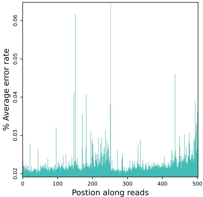
Error rate distribution along reads (R20109)
